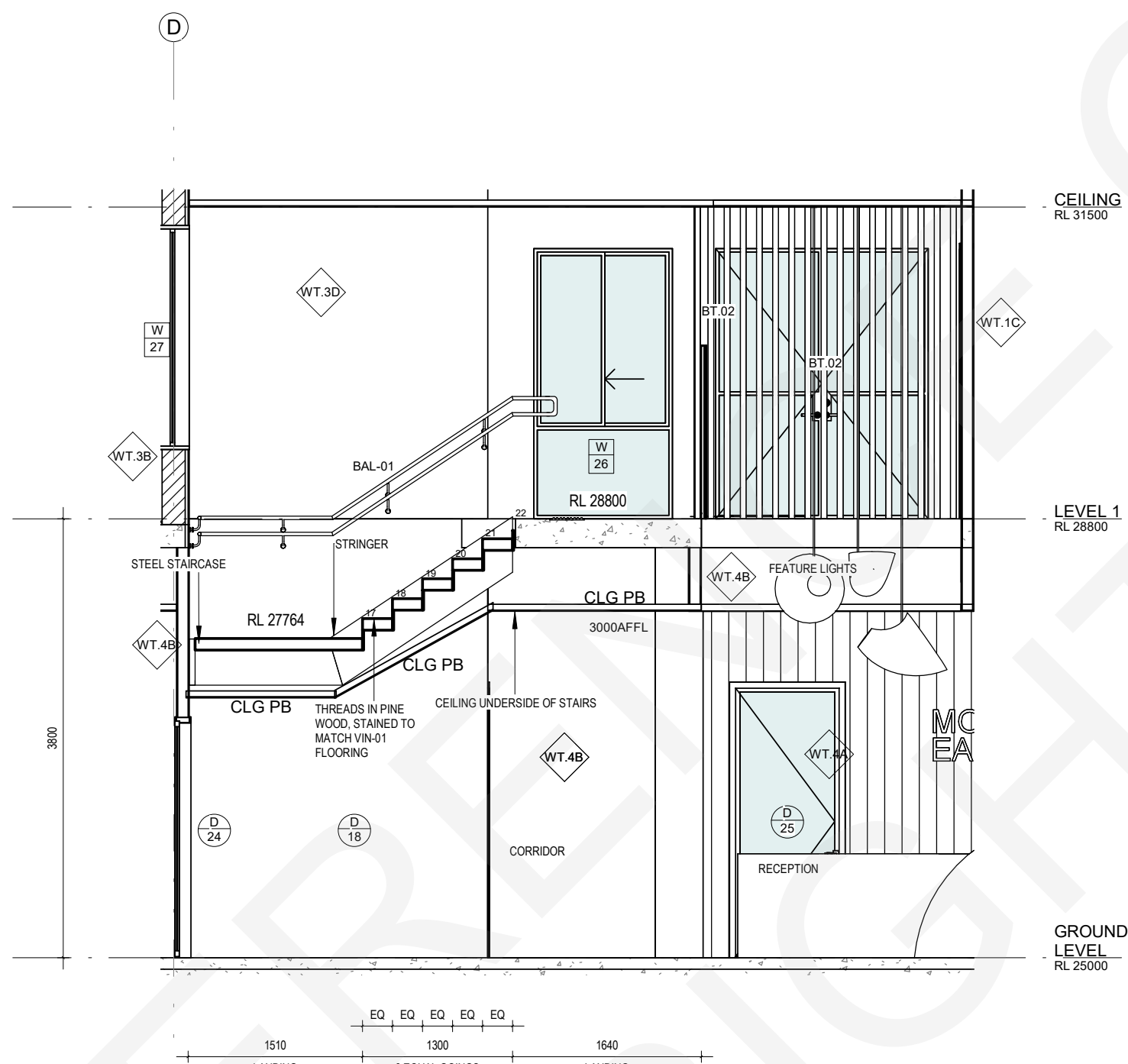
INTERNAL STAIRWAY ELEVATION 02 1:50 REFER 4 - BA.400
