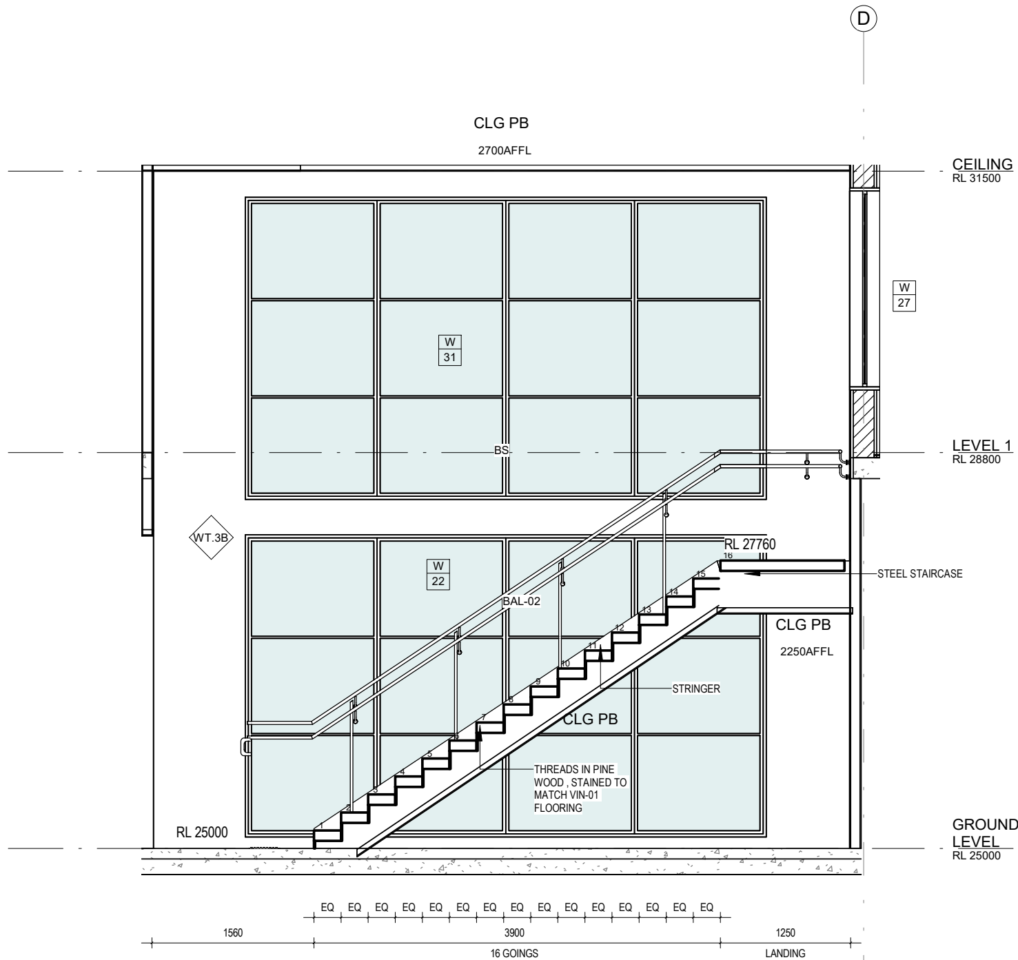
INTERNAL STAIR ELEVATION 01 1:50 REFER 3 - BA.400
