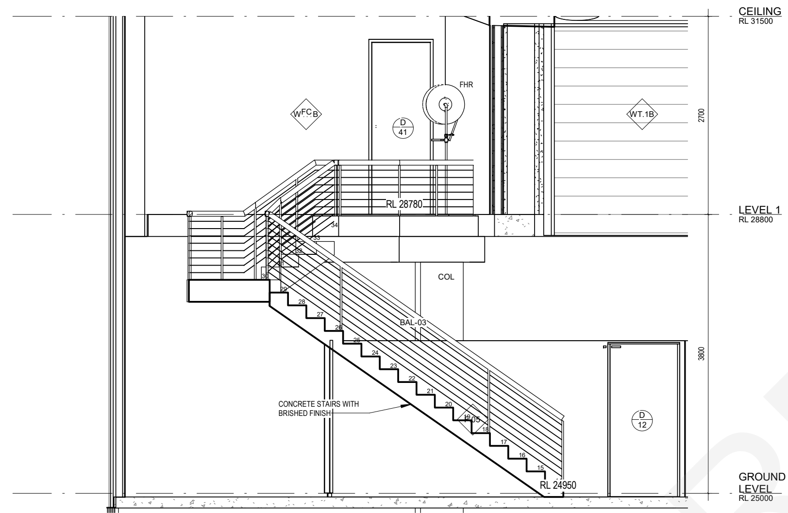
FIRE STAIRCASE -ELEVATION 1 1:50 REFER 4 - BA.106
