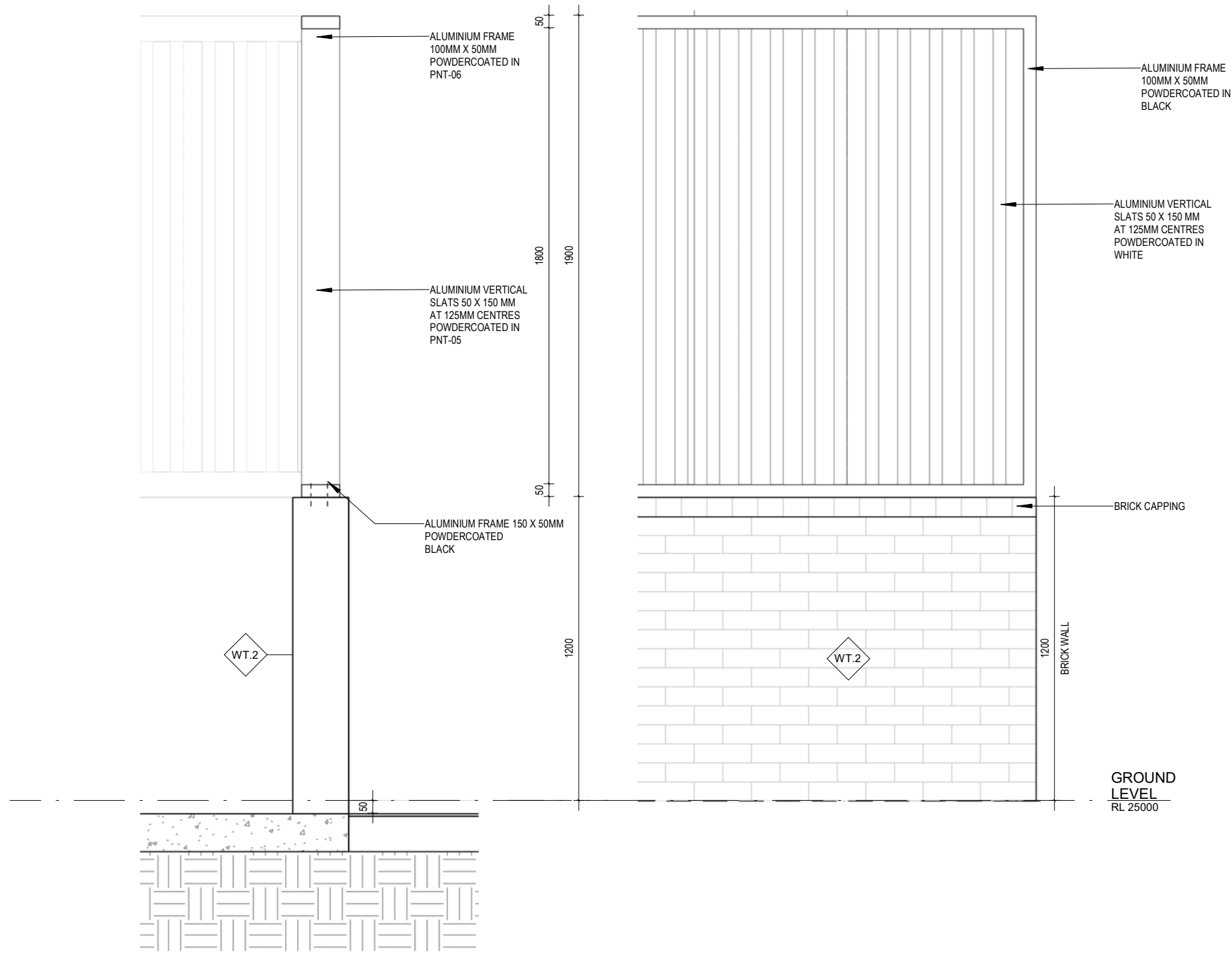
F.01 FENCE SECTION DETAIL
