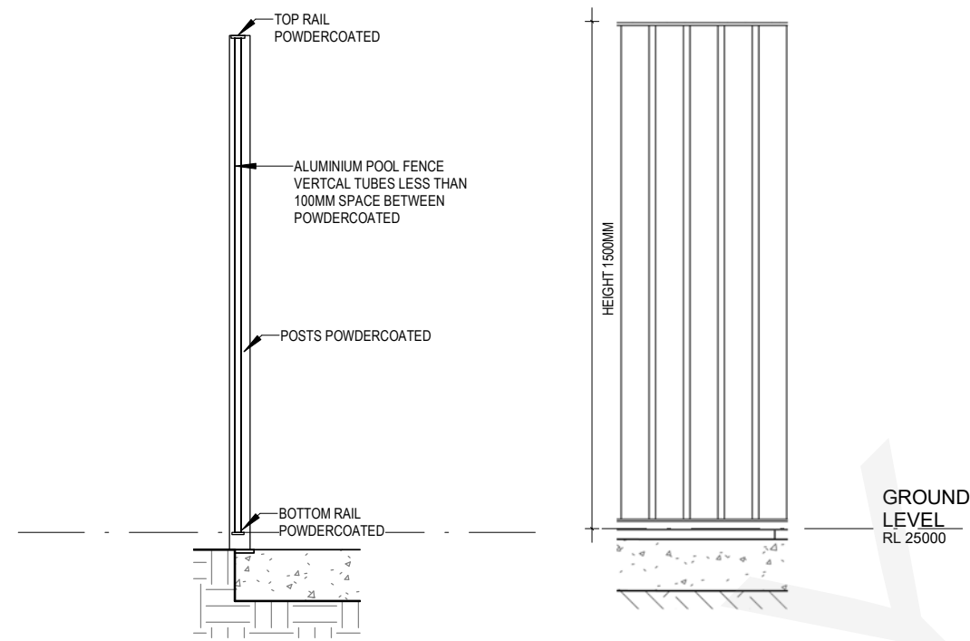
F.03 DETAIL SECTION
