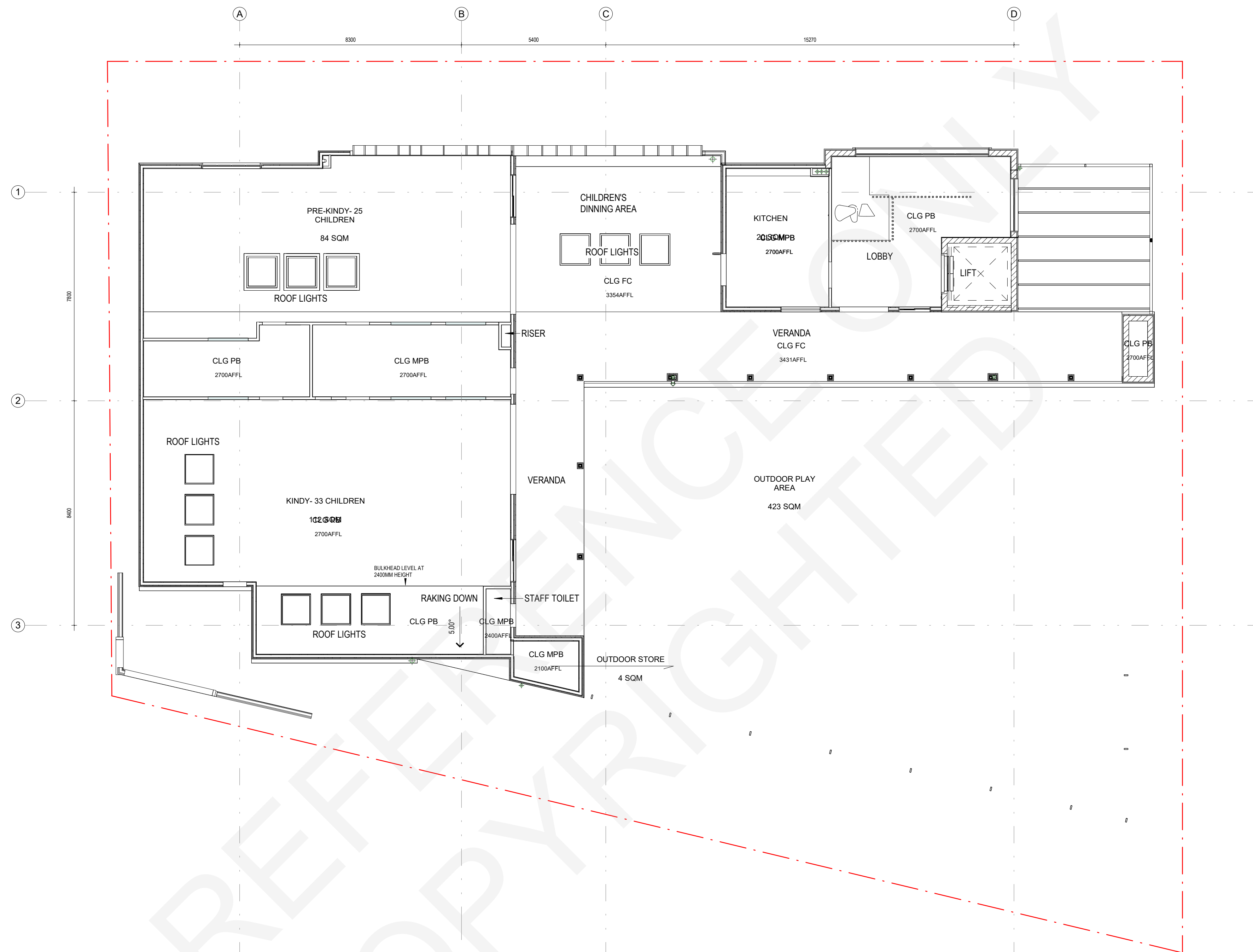
PROPOSED RCP_LEVEL 1 1:100
