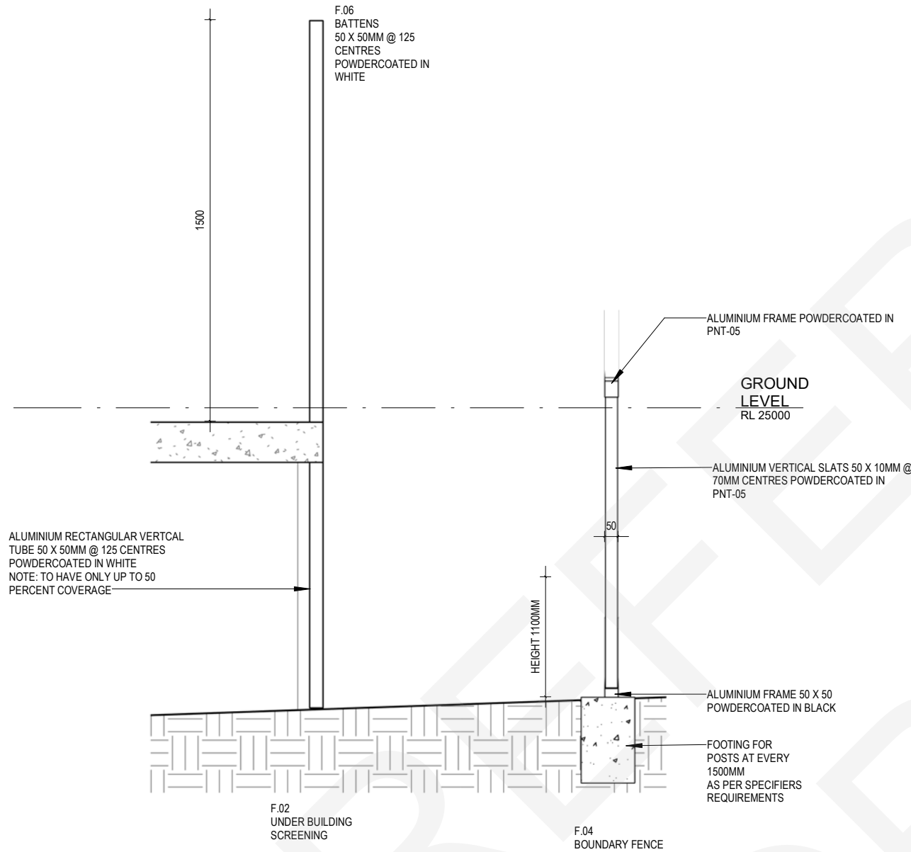
F.02 and F.04 DETAIL SECTION
