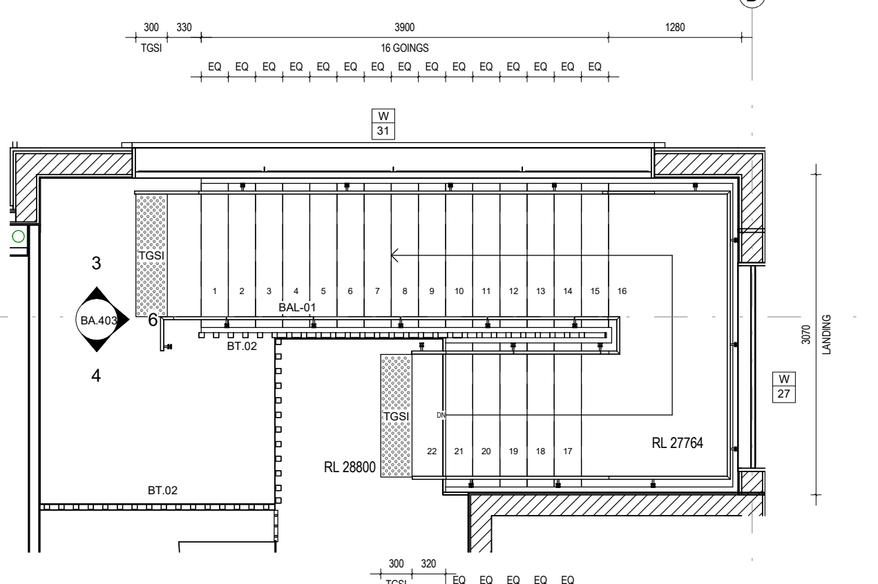
INTERNAL STAIR- FIRST FLOOR LEVEL 1:50 REFER 2 - BA.104
