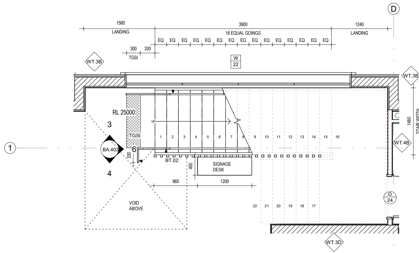
INTERNAL STAIR - GROUND FLOOR LEVEL 1:50 REFER 1 - BA.103
