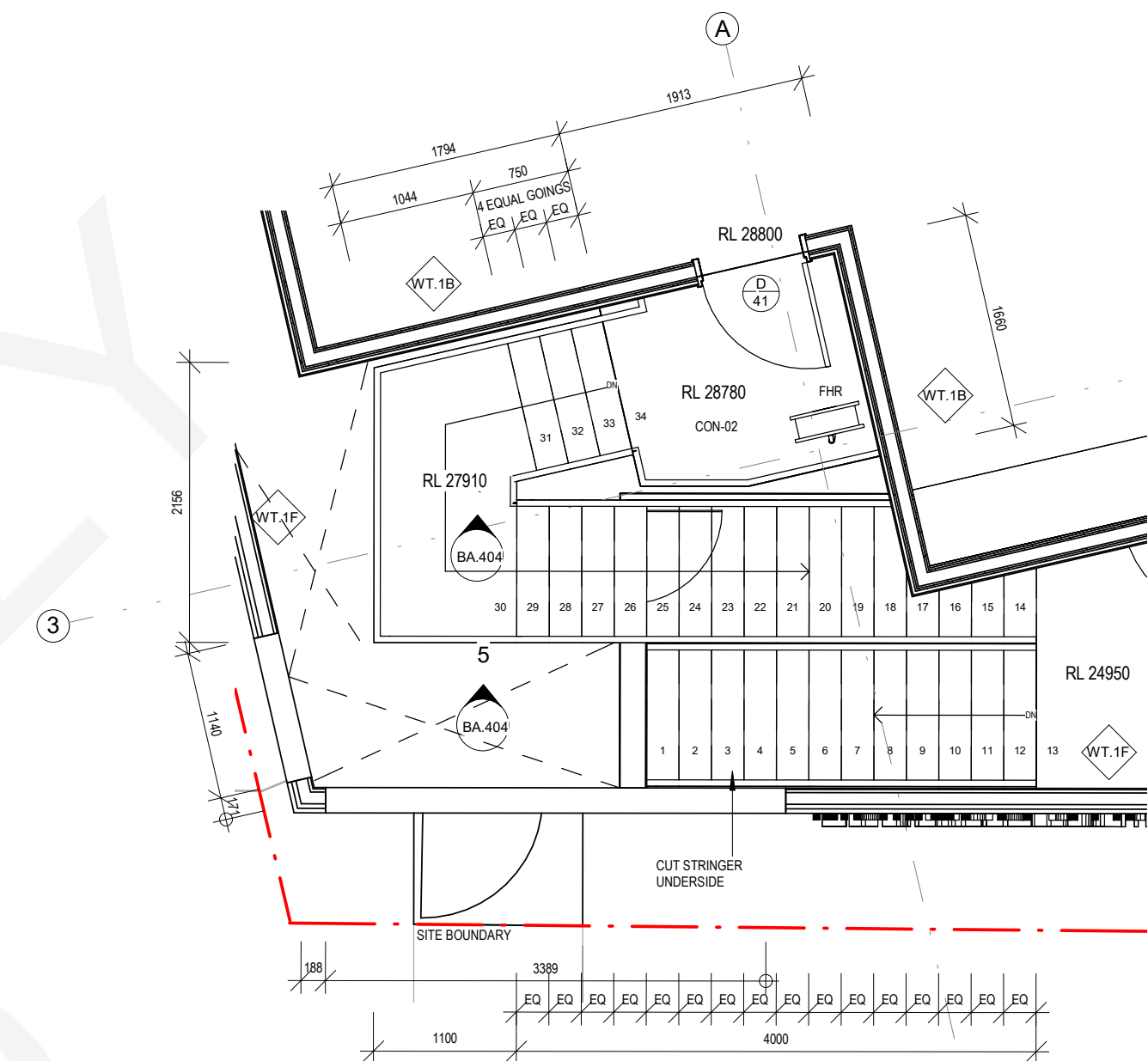
FIRE STAIRWAY- LEVEL 1 FLOOR PLAN 1:50 REFER 3 - BA.104
