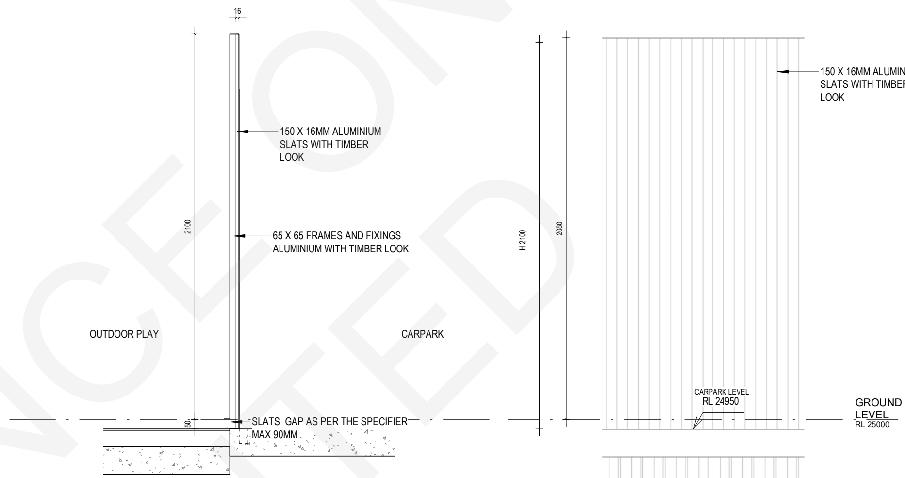
F.05 DETAIL SECTION
