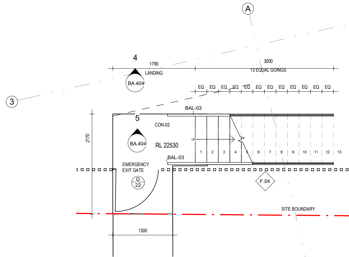
FIRE STAIRWAY DETAIL- LOWER GROUND FLOOR PLAN - Callout 1 1:50 REFER 2 - BA.103
