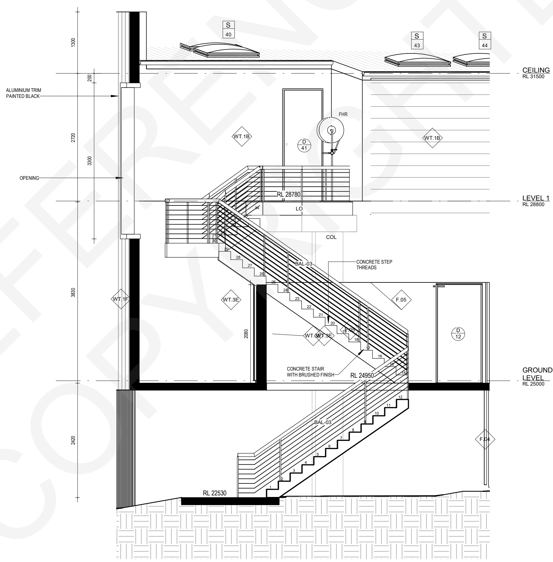
FIRE STAIRCASE -ELEVATION 01 1:50 REFER 5 - BA.106
