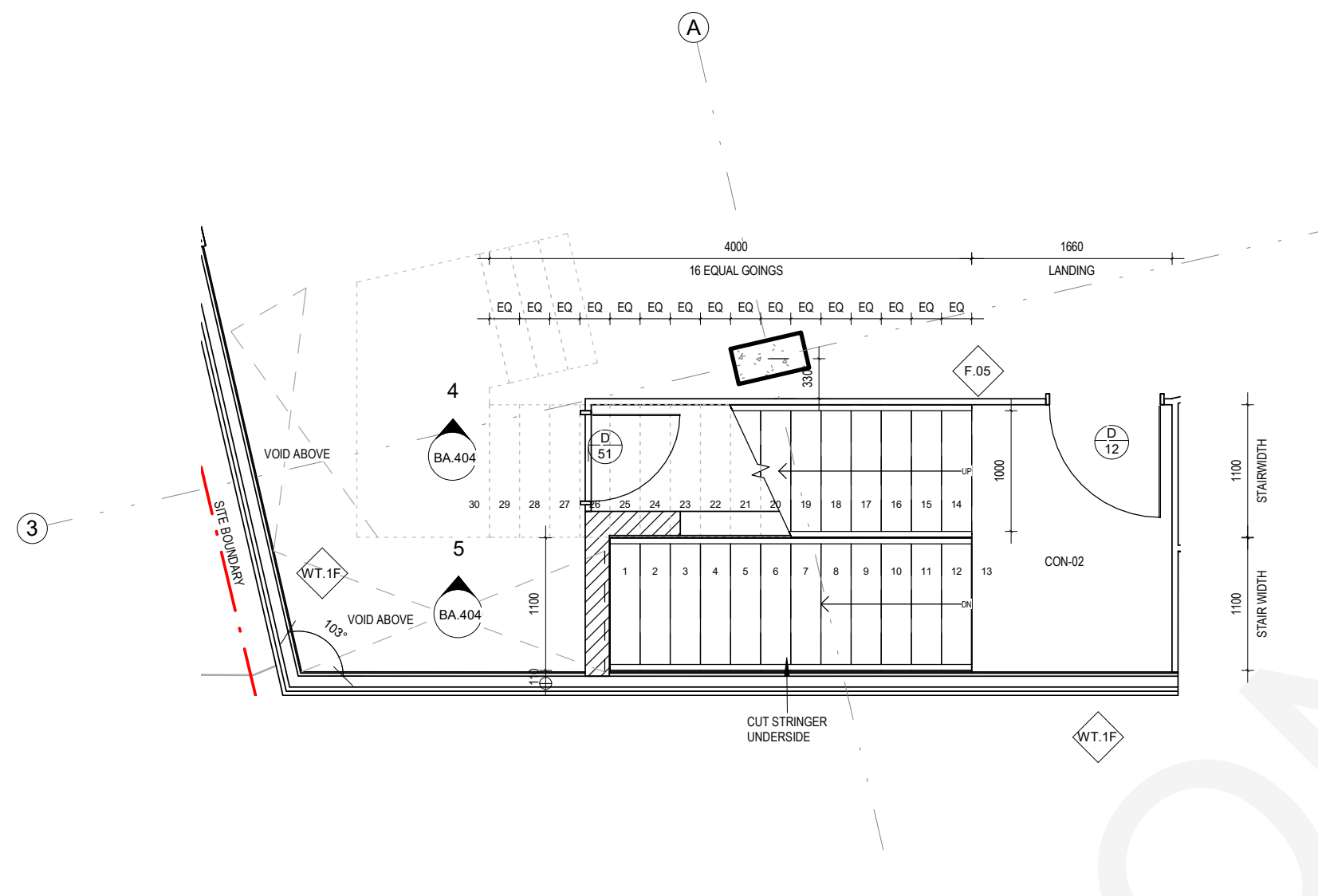
FIRE STAIR DETAIL_ GROUND FLOOR 1:50 REFER 1 - BA.103
