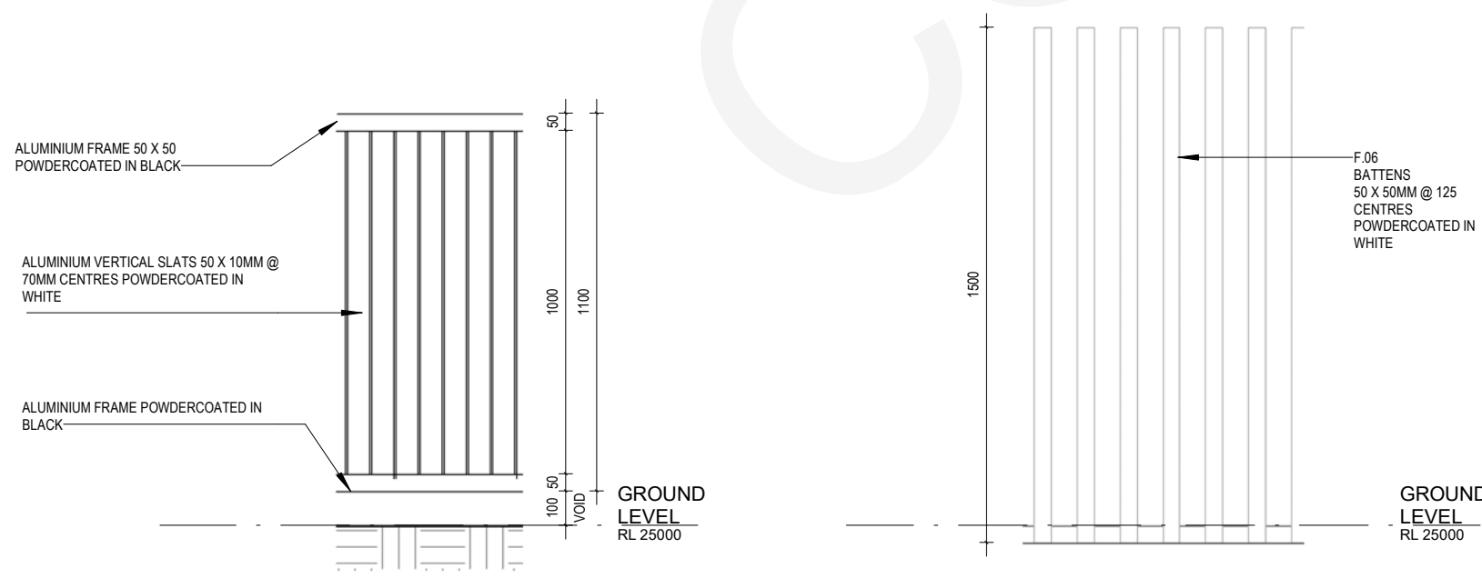
F.04 FENCE DETAIL ELEVATION
